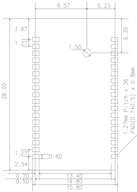
[BCD210SU, SC]
